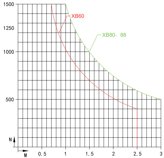
60、80、88系列中重型悬臂承重受力图 Bearing and force diagram for 60、80、88 series medium sized and heavy duty cantilever walls
