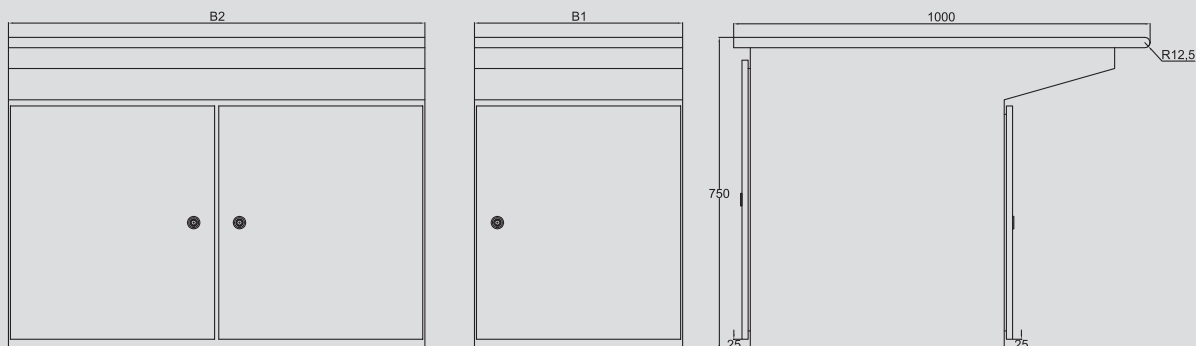
AP series detail drawing
