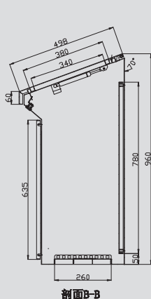
APXM series detail drawing
