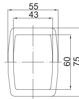
5575铝管规格表 (配5575中型悬臂) : 5575 aluminum spec sheet (with medium-sized cantilever 5575):
