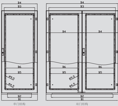
AK/BAK series detail drawing
