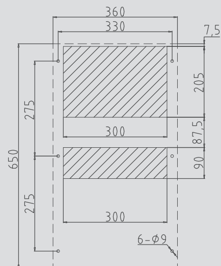
WSKT1000无水空调开孔图 WSKT1000 portiforium drawing
